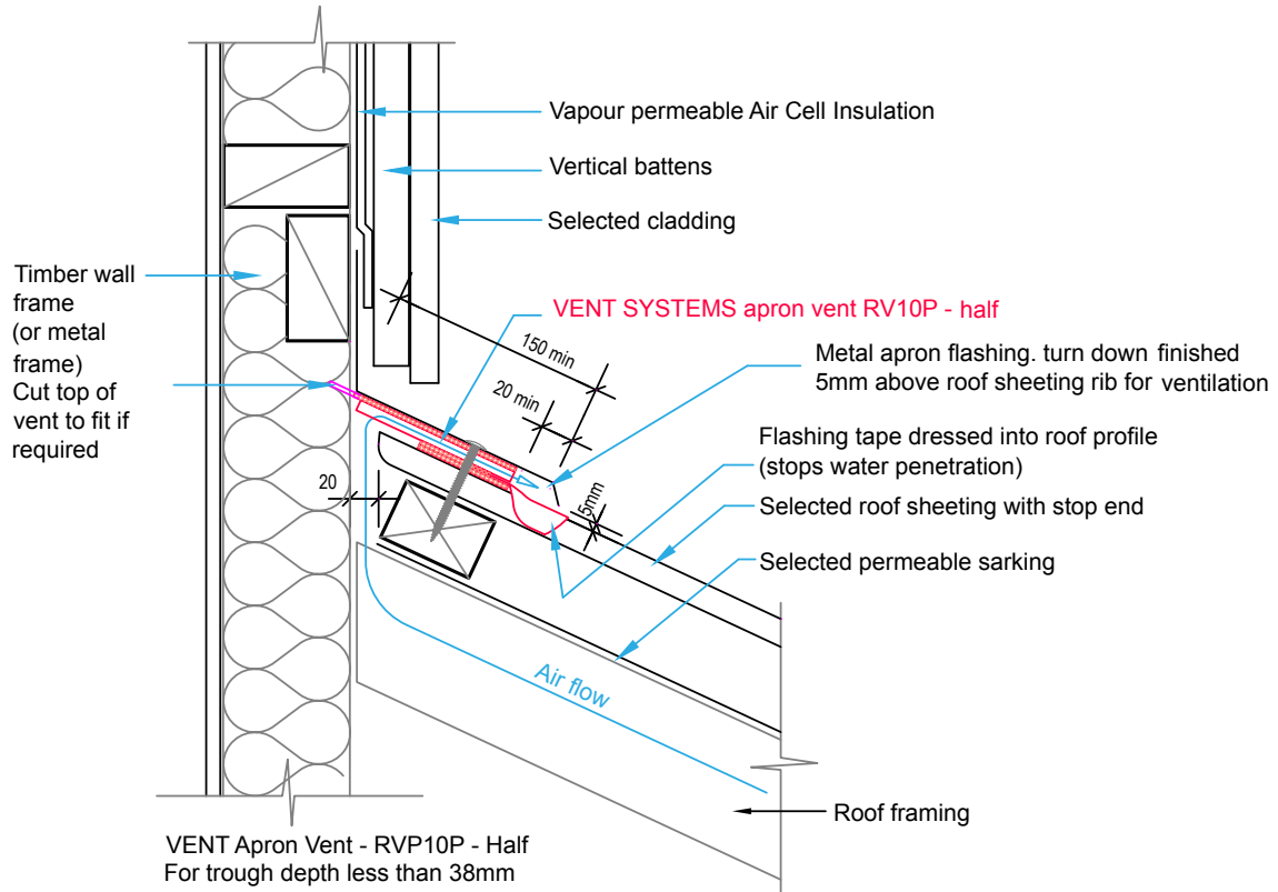
Fig C: Dimensions
