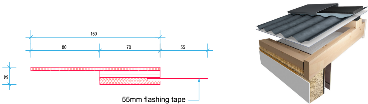
VENT SYSTEMS Apron Vent - RV10P - Half (free air flow 8,000mm 2 per lineal metre)
