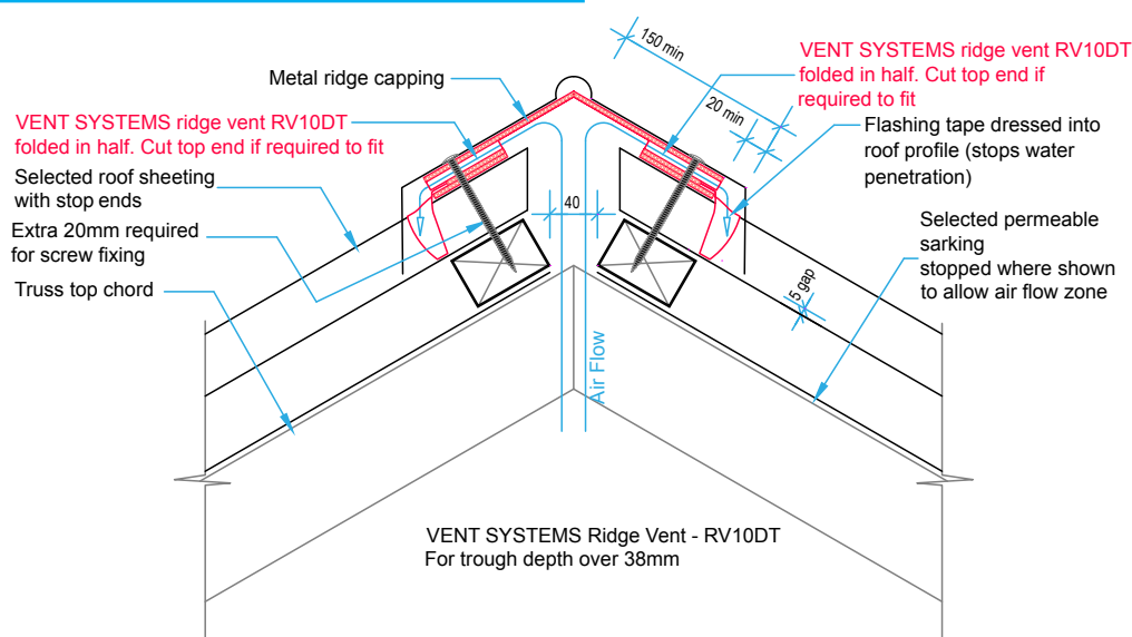
Fig C: Dimensions
