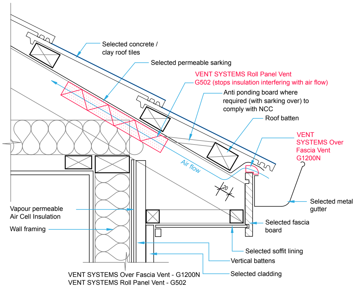
Figure A: VENT System G1200N with VENT Systems Eaves Comb Filler - G1275
